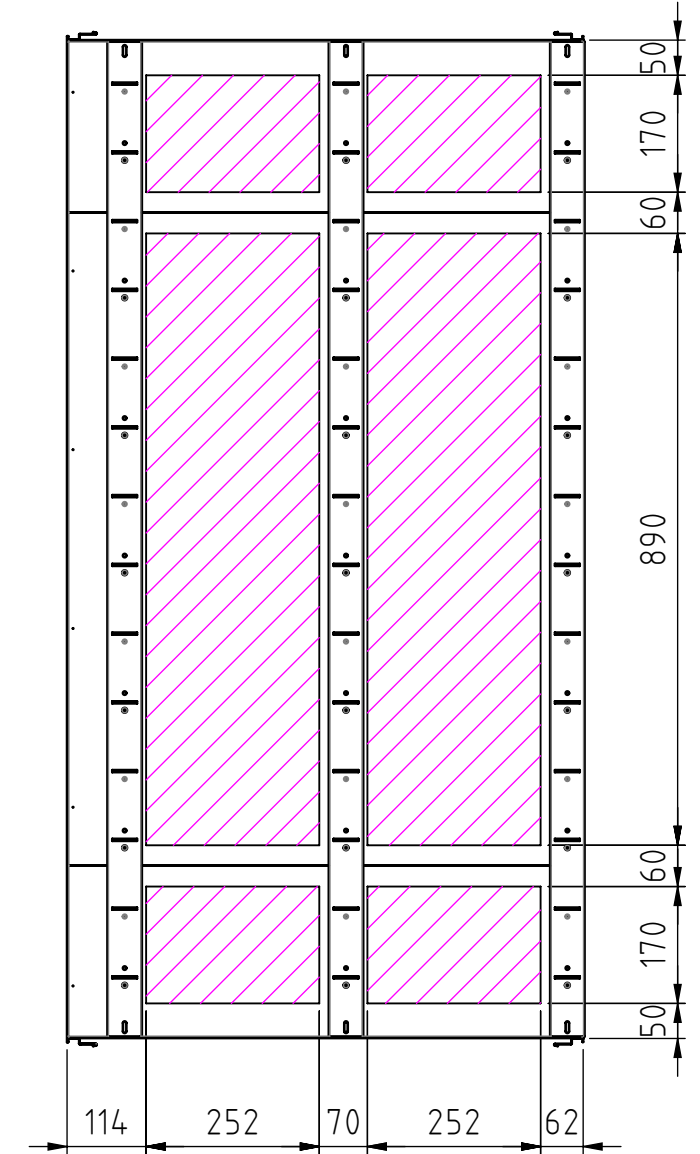
B-B View from inside right
