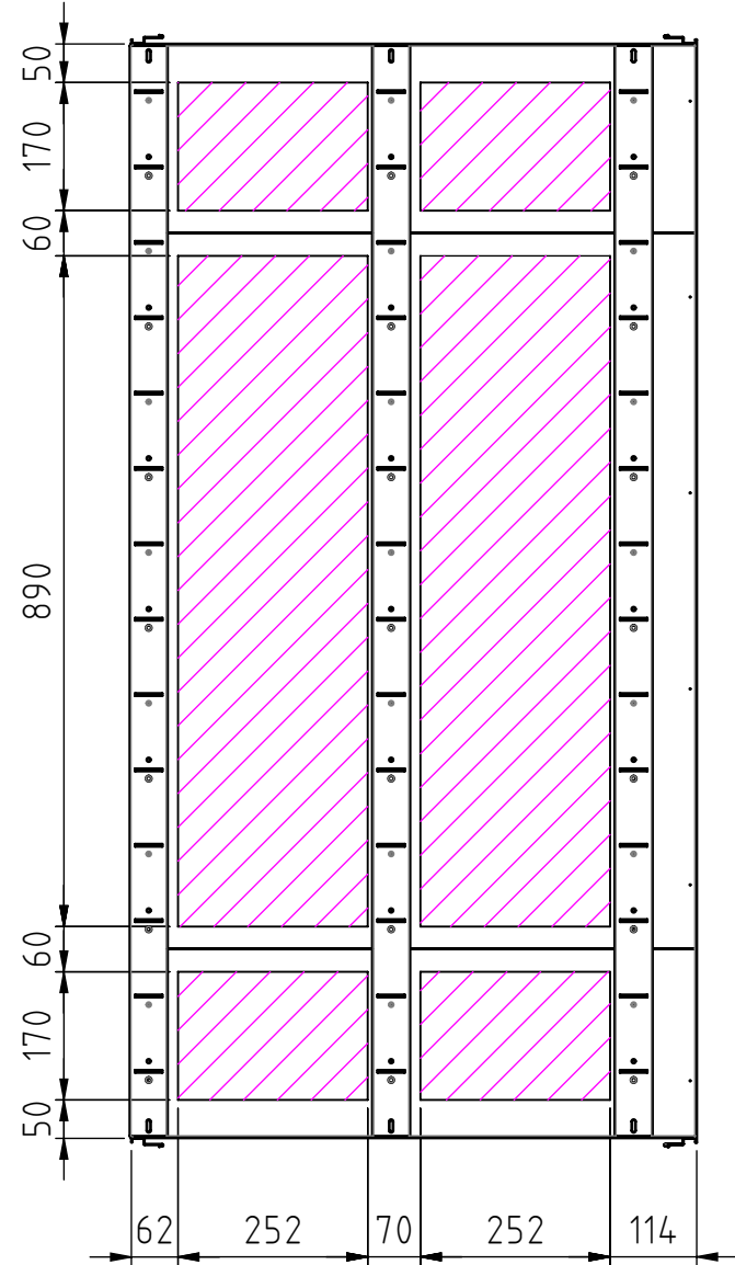
A-A View from inside left
