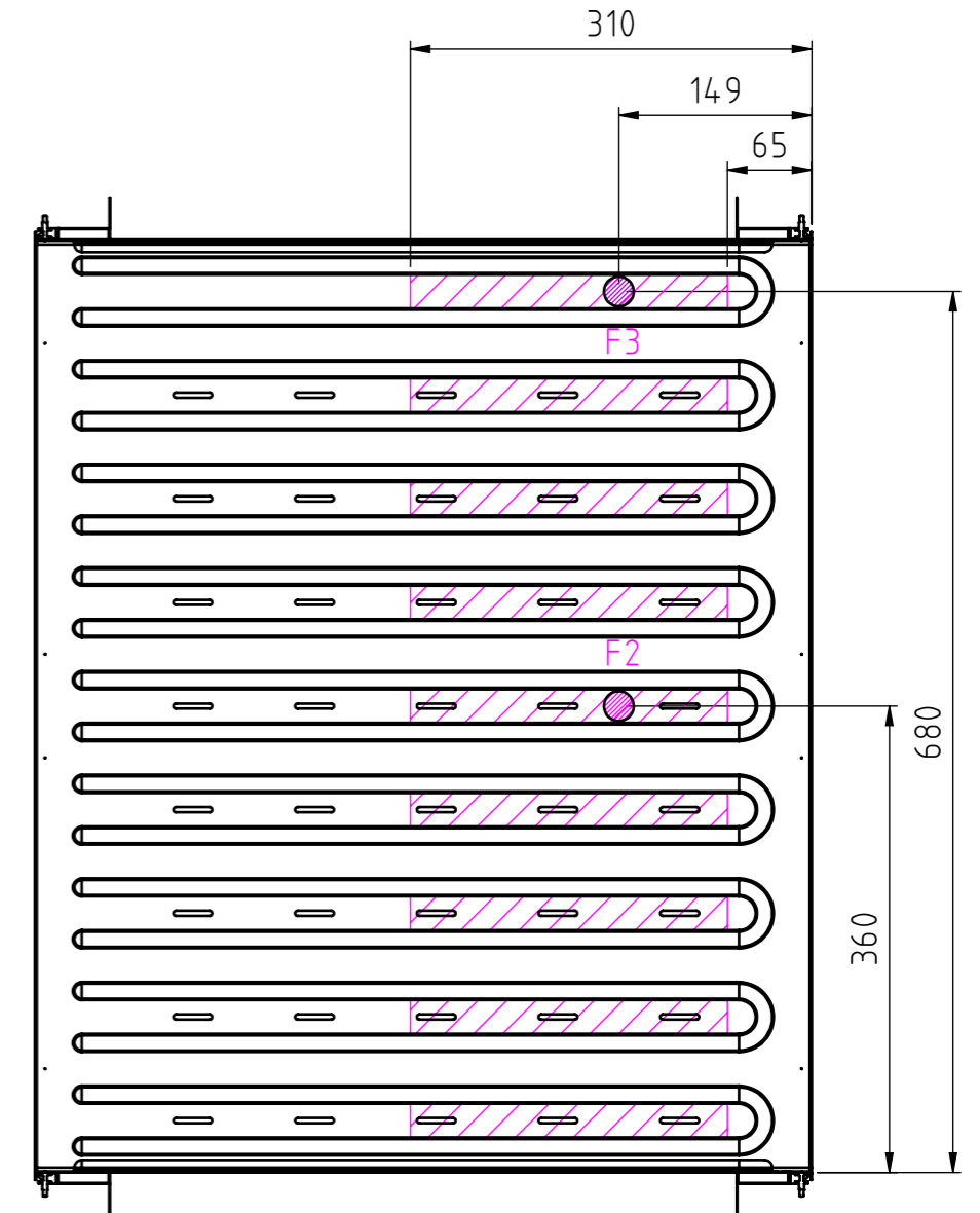
B-B 1:6 view from inside right
