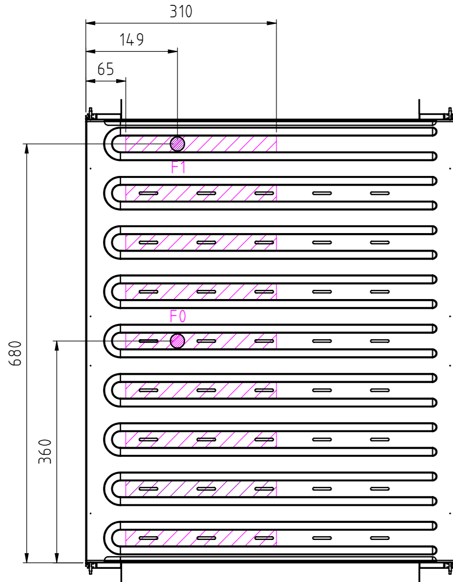
A-A 1:6 view from inside left
