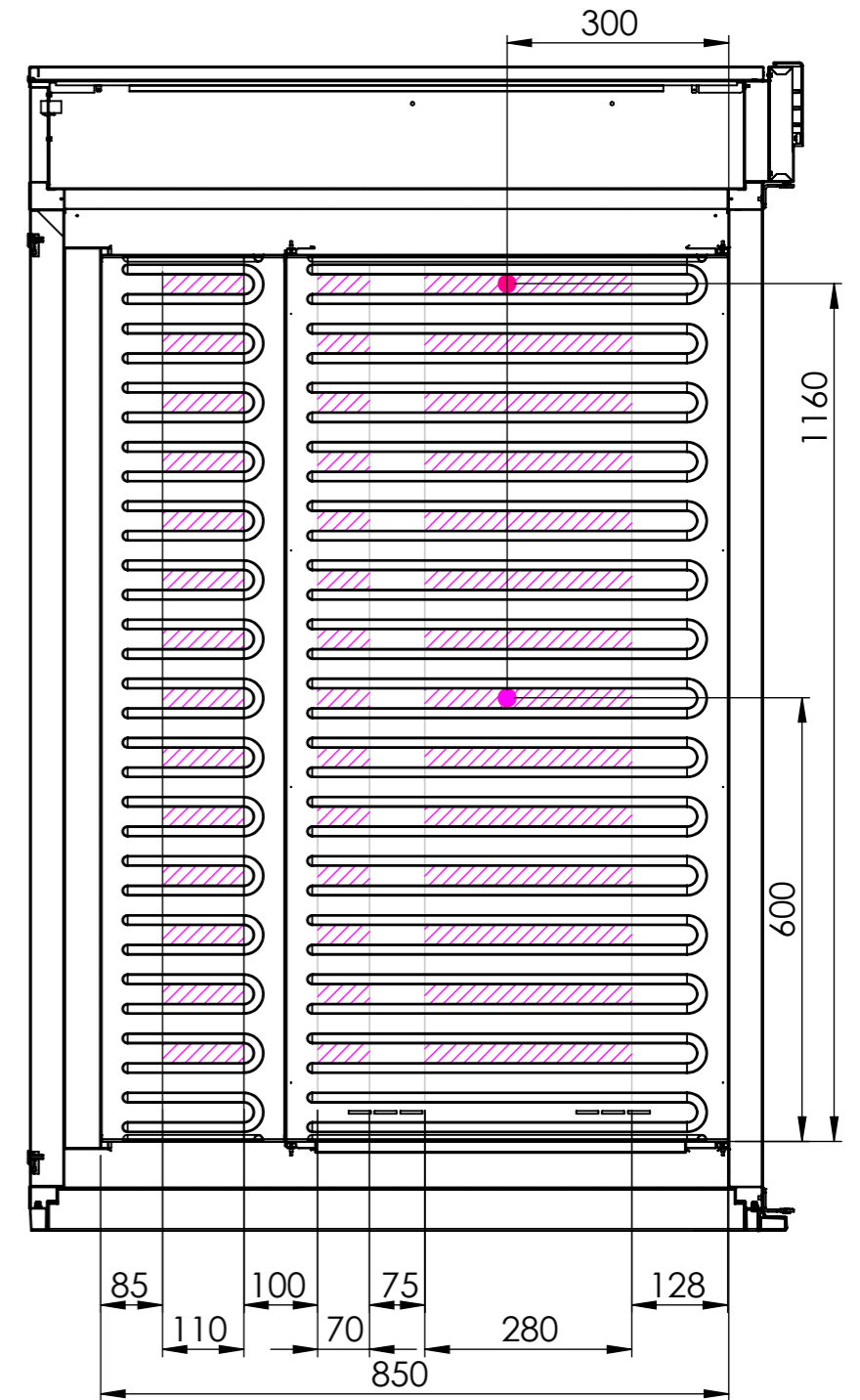
B - B view from inside right
