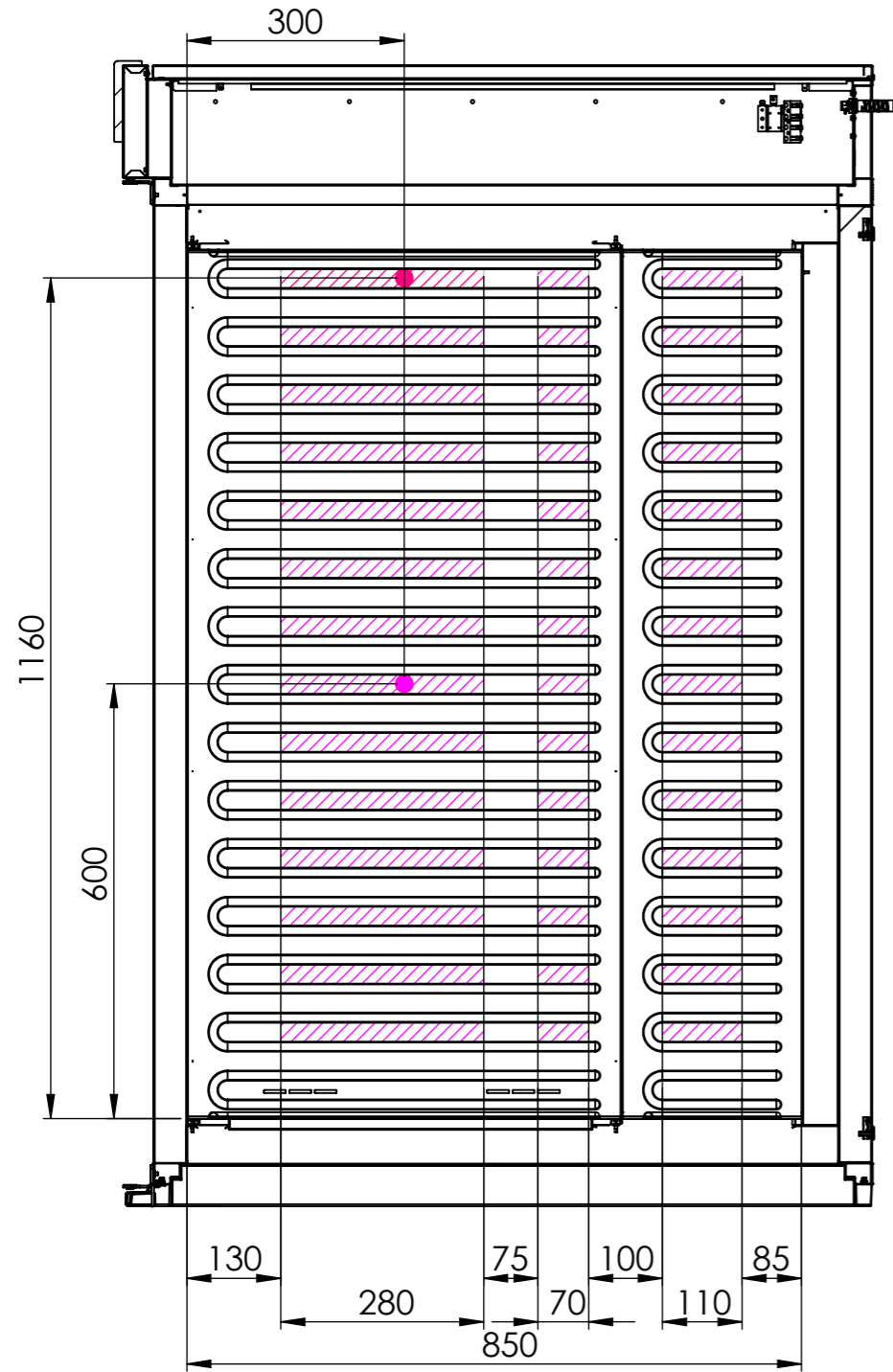
A - A view from inside left
